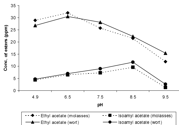
Fig. 3. The effect of pH on ester synthesis.
